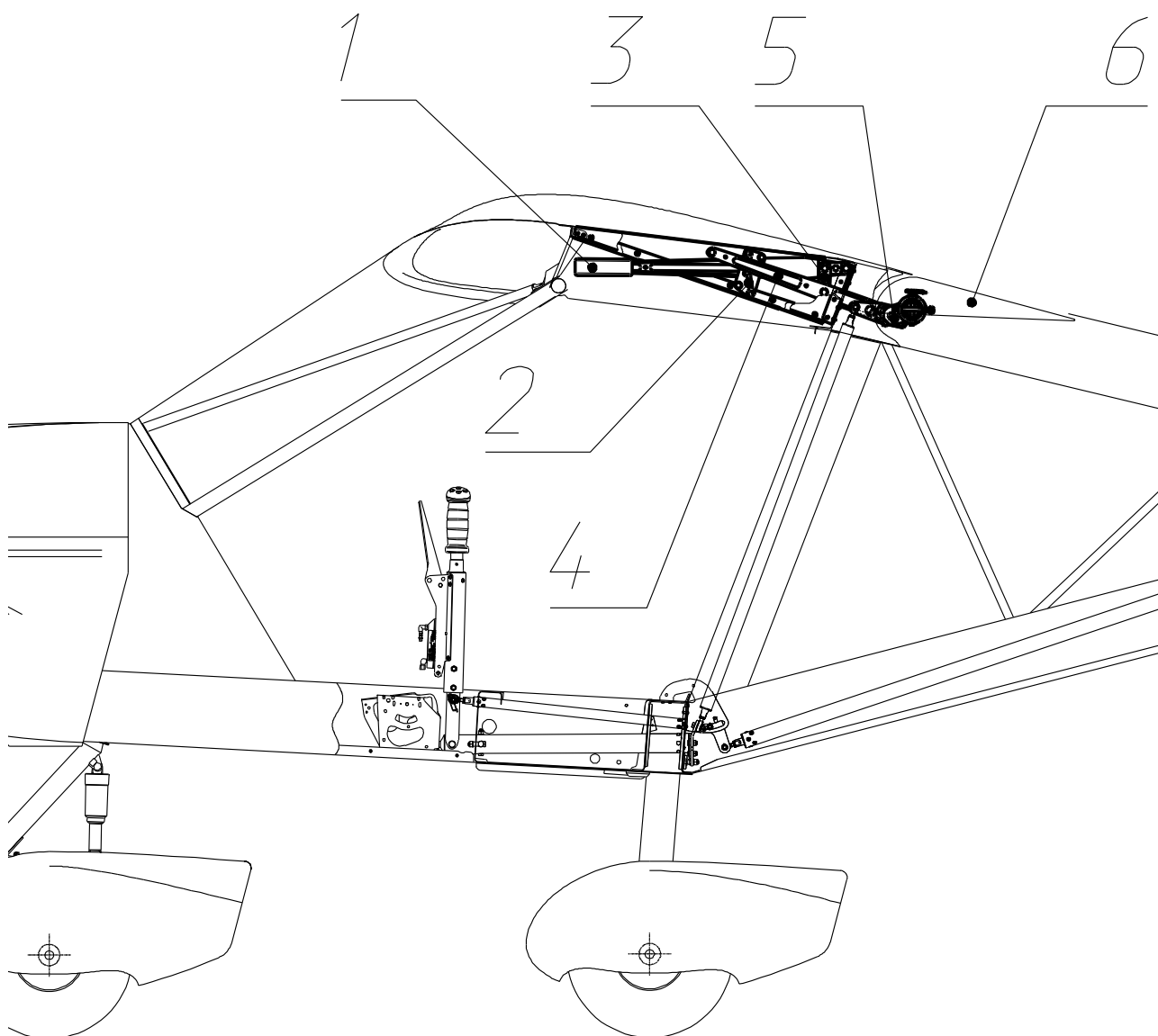
Fig. 8. Flap extension mechanism
