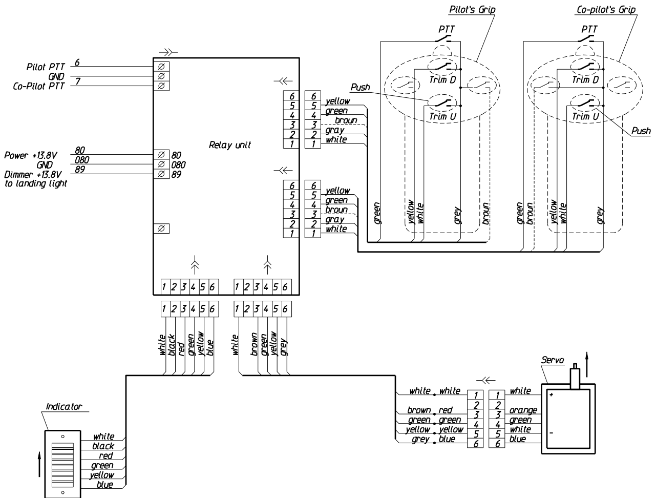
Fig. 16. Wiring diagram for installation of PTT and trimmer control buttons
