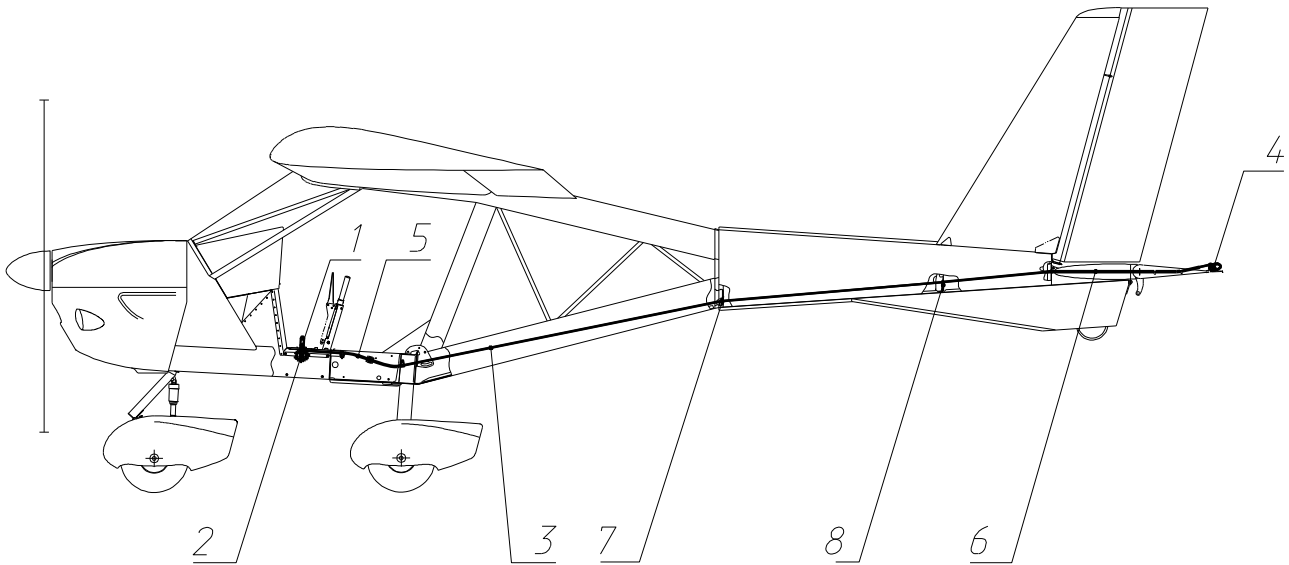
Fig. 5 Elevator trim tab control system
